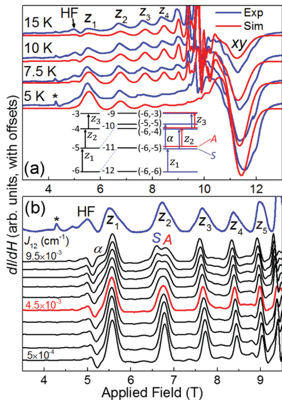
Fig. 10 (a) Experimental (Exp) and simulated (Sim) powder HFEPN spectra of 3.5py·H 2 O at a frequency of 270 GHz, plotted as dI/dH ( I = transmitted intensity) for temperatures in the range from 5 to 15 K. The resonances labeled z_1 to z_4 correspond to the parallel ( z -) components of the powder pattern, xy correspond to the perpendicular components, and HF is a half field transition (see main text for explanation); the feature labeled with an asterisk (*) corresponds to a known O 2 impurity in the sample holder. The inset schematically depicts the lowest lying energy levels appropriate to the parallel resonances. On the left are the uncoupled states associated with each individual S = 6 Mn 3 SMM, labeled according to m_S value, with the m_{S1}, m_{S2} transitions corresponding to resonances z_1 to z_3 labeled. The middle panel shows the levels associated with the uncoupled dimer, labeled according to |m_{S1}, m_{S2}\rangle ; as can be seen, the new states are generated simply by exciting one of the spins, thereby translating (dashed lines) the overall energy of the dimer accordingly. The right panel depicts the fully coupled energy levels, labeled according to |m_{S2}, m_{S1}\rangle , where the blue and red states respectively correspond to the symmetric ( S ) and antisymmetric ( A ) combinations of |m_{S1}, m_{S2}\rangle and |m_{S2}, m_{S1}\rangle . (b) Simulations of the 10 K spectrum as a function of the exchange coupling parameter, J_{12} (in steps of 10^{-3} cm -1 , see legend). The linewidth is reduced from the best simulations in (a) so that it is possible to resolve additional resonances that emerge due to the exchange coupling, i.e. , \alpha and the S and A z_2 resonances. The red simulated spectrum corresponds to the value of J_{12} deduced from magnetic hysteresis experiments and the value used for the simulations in (a).
