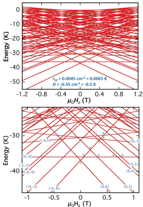
Fig. 8 (Top) Spin state energies vs. applied dc field plot for 3\cdot 3\text{py}\cdot 12\text{CH}_2\text{Cl}_2 constructed with J = +4.5 \times 10^{-3} \text{ cm}^{-1} ( \hat{H} = -2J_{12}\hat{S}_1\hat{S}_2 convention) and D = -0.35 \text{ cm}^{-1} to simulate the positions of the avoided level crossings that lead to the experimentally observed QTM step positions in the hysteresis loops of Fig. 6. (Bottom) Expansion showing only the lower energy spin states populated at very low temperature, and the avoided level crossings relevant to the hysteresis loops in Fig. 6 when the field is swept from -1.2 \text{ T} to +1.2 \text{ T} . The green numbers 1 to 9 are the crossings listed in Table 3. Spin states are labelled in blue as (m_{S1}, m_{S2}) for the two \text{Mn}_3 units. See the text for the discussion of the avoided level crossings leading to the observed QTM steps in Fig. 6.
