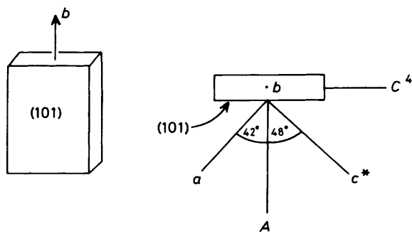
Figure 1. Crystal morphology and relationship between crystal axes and axes used for e.s.r. measurements
