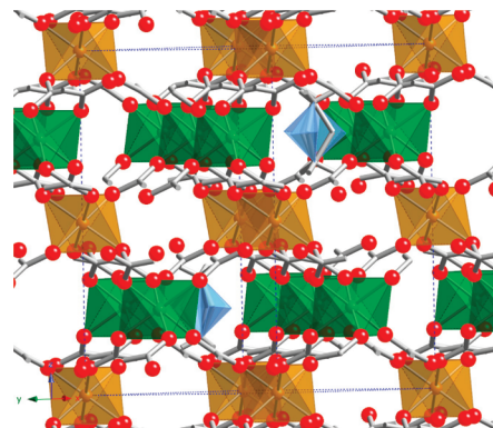
Figure 2. Polyhedral representation of the layered structure of 3 , with \text{Fe}(\text{II}) in green, \text{Fe}(\text{III}) in blue, and \text{N} in blue (only two representative cations are shown).
