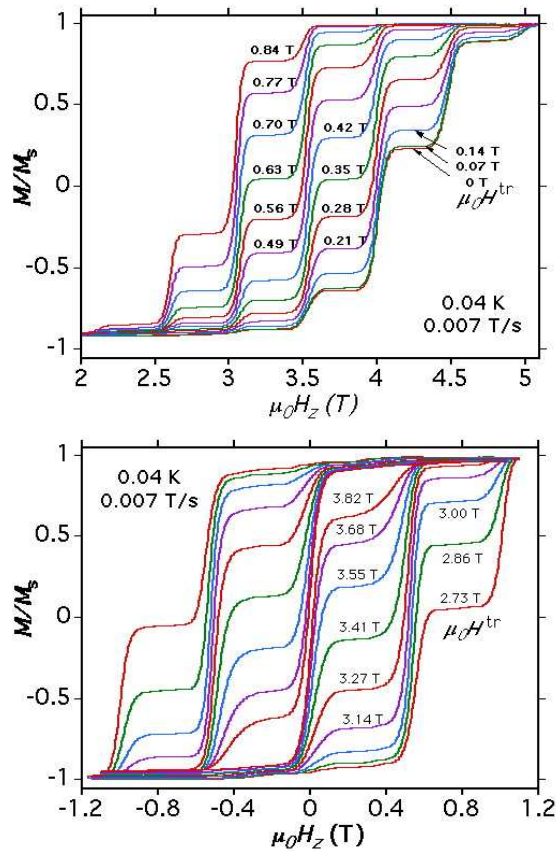
FIG. 4: (Online color) (a and b) Normalized magnetization along the c -axis of the crystal versus applied field along the c -axis for several constant transverse fields H_{tr} . Although the transverse fields increase the tunnel rates, no significant broadening of the resonance fields is observed.
