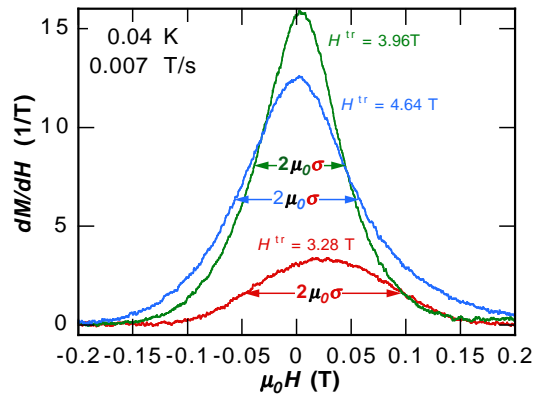
FIG. 5: (Online color) Derivative dM/dH of three hysteresis curves at the zero field resonance for a field sweep from negative to positive fields. The definition of the width \sigma at the half-width-at-half-maximum is shown.
