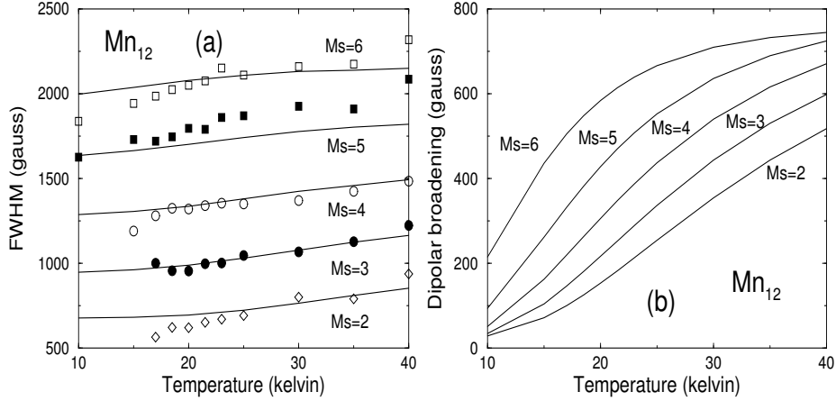
Figure 2: (a) Calculated (curves) and measured (symbols) FWHM vs temperature at \nu = 189.123 GHz for \text{Mn}_{12} . Here the D strain ( \sigma_D \sim 0.018D ), g strain ( \sigma_g \sim 0.002g ), and the dipolar interactions ( \Gamma = 203 \text{ G}^2 ) are included in the calculated linewidths. (b) Calculated FWHM caused by the dipolar interactions only, shown vs temperature, at \nu = 189.123 GHz with \Gamma = 203 \text{ G}^2 for \text{Mn}_{12} . The examined temperature range for \text{Mn}_{12} is from 10 K to 40 K. Cited from Ref.[20].
