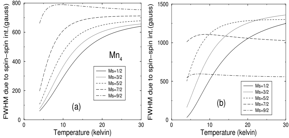
Figure 3: (a) Calculated linewidths due to the exchange and dipolar interactions only vs temperature at \nu = 138 GHz for Mn_4 . Here we use the exchange coupling constant J = -40 G, \Lambda = \sum'_{ij} J_{ij} A_{ij}/N = -1854.8 G 2 , and \Gamma = \sum'_{ij} A_{ij}^2/N = 344 G 2 . (b) The same linewidths as in (a) when the sign of J is flipped and the other parameter values are kept the same.
