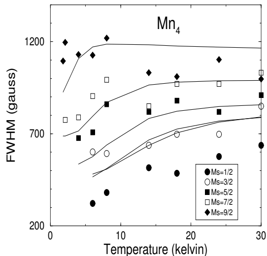
Figure 4: Calculated (curves) and measured (symbols) FWHM vs temperature at \nu = 138 GHz for \text{Mn}_4 . Here we use \sigma_D = 0.01D , \sigma_g = 0.004g , J = -40 G, \Lambda = \sum'_{ij} J_{ij}A_{ij}/N = -1854.8 G 2 , and \Gamma = \sum'_{ij} A_{ij}^2/N = 344 G 2 . The solid curves, from bottom to top, correspond to M_s = 1/2, 3/2, \dots, 9/2 .
