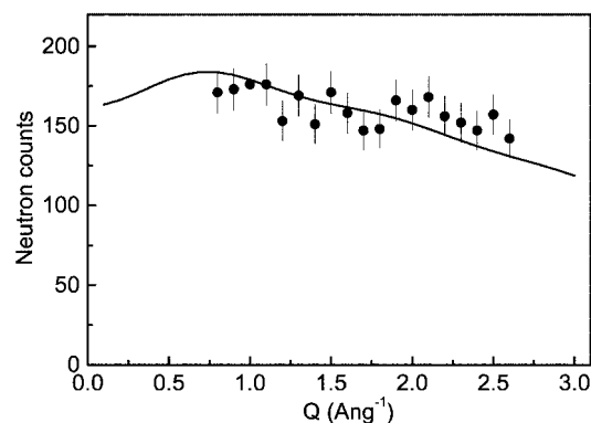
Fig. 5. Q -dependence of peak (I) at \hbar\omega \approx 1.50 \text{ meV} measured at 1.5 K on the triple-axis spectrometer Drüchäl (PSI, Switzerland) with final energy E_f = 4.5 \text{ meV} . The solid line is a calculation based on Eq. (1) with J_b = -4.80 \text{ meV} , J_{w1} = +0.10 \text{ meV} , J_{w2} = -0.10 \text{ meV} and D = -0.47 \text{ meV} .
