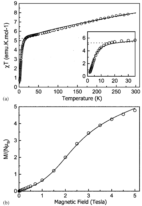
Fig. 2. (a) Magnetic susceptibility measured under a static magnetic field of H = 0.1 T. (b) Magnetization curve at T = 1.8 K. In both panels, continuous lines are calculated curves based on the model discussed in the text. The best fit to the susceptibility and magnetization data was obtained for J_b = -4.80 \pm 0.10 meV, J_{w1} = +0.10 \pm 0.002 meV, J_{w2} = -0.10 \pm 0.002 meV, D = -0.47 \pm 0.01 meV and g = 1.94 \pm 0.03 . The dotted line corresponds to the parameters proposed in Ref. [21]; J_b = -3.35 meV, J_w = J_{w1} = J_{w2} = -0.05 meV and g = 1.87 .
