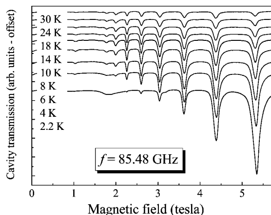
Fig. 4. Hard axis spectra for SB4. The temperatures and the frequency are indicated in the figure; the traces are offset for clarity.
