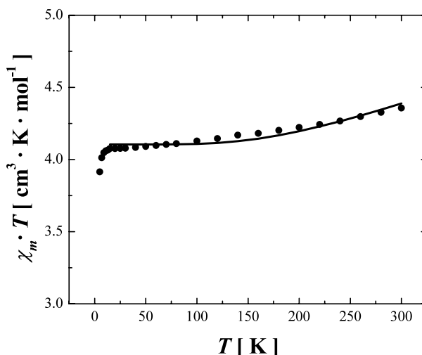
Fig. 2. Plot of \chi_M T versus temperature where \chi_M is the molar susceptibility. The solid line represents the best least-squares fit of the data, see the text for details.
