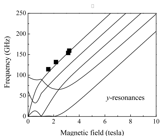
Fig. 8. Zeeman diagram of the spin Hamiltonian associated with the S = 5/2 ground state of complex 1 with the magnetic field oriented in the y direction. The solid lines represent the energy spectrum obtained from a best fit of the y resonances.
