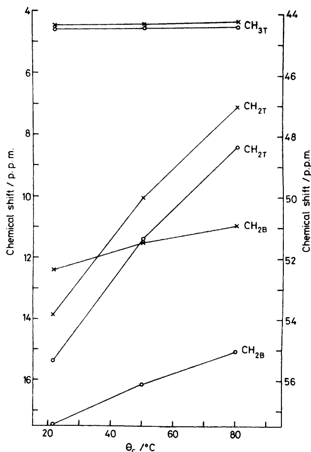
FIGURE 9 Temperature dependences of the ^1\text{H} n.m.r. chemical shifts of [\text{Fe}_6\text{M}_2\text{S}_8(\text{SEt})_6]^{3-} [ \text{M} = \text{Mo} ( \circ ) or \text{W} ( \times )] complexes (the right-hand scale refers to \text{CH}_{2\text{T}} protons)
