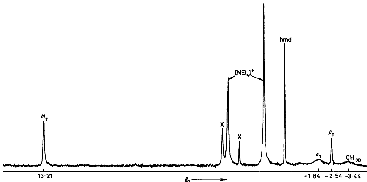
FIGURE 5 300 MHz ^1\text{H} n.m.r. spectrum of [\text{Fe}_6\text{W}_2\text{S}_8(\text{SPh})_6(\text{OMe})_3]^{3-} in [\text{H}_6]\text{dmsO} at ca. 23 ^\circ\text{C} (solvent peaks marked by \times )
