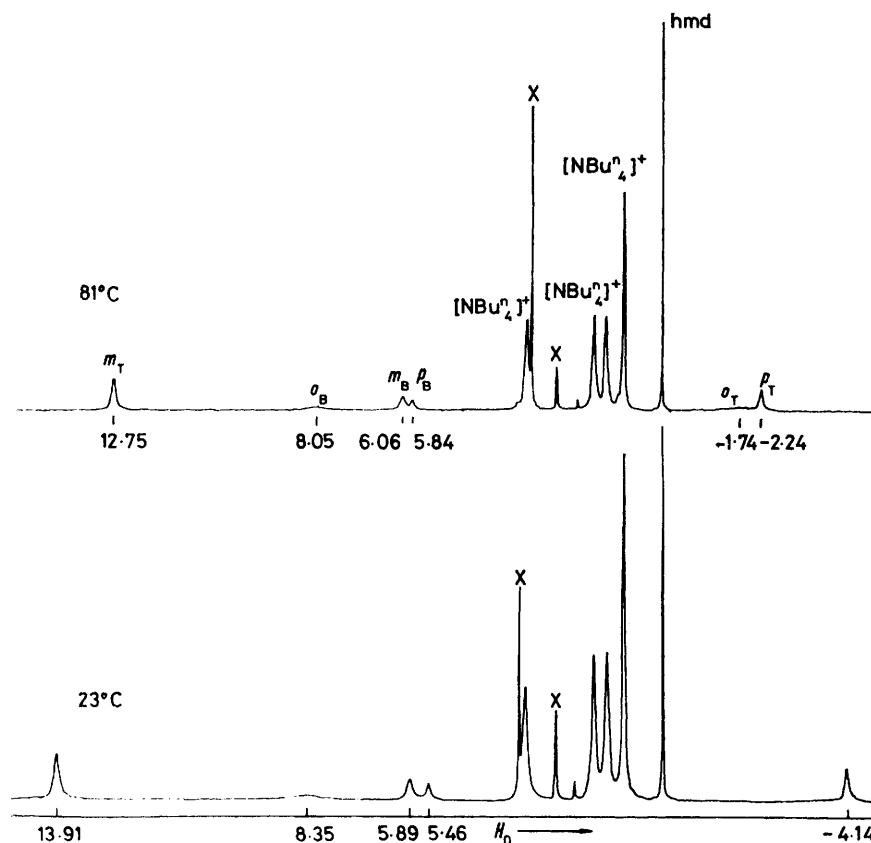
FIGURE 2 300 MHz ^1\text{H} n.m.r. spectra of [\text{Fe}_6\text{Mo}_2\text{S}_8(\text{SPh})_6]^{3-} in [\text{}^2\text{H}_6]\text{dmsO} (solvent peaks marked by X)
