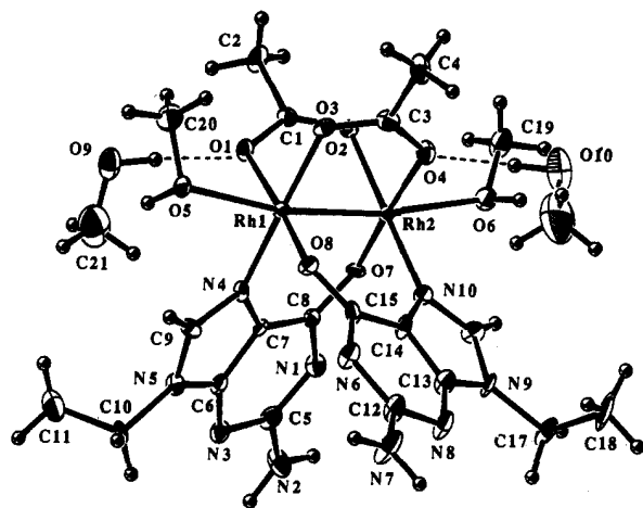
Figure 1. ORTEP drawing of a molecule of \text{Rh}_2(\text{O}_2\text{CCH}_3)_2(9\text{-EtG})_2 \cdot 2\text{MeOH} with thermal ellipsoids drawn at the 30% probability level. Selected bond lengths (Å) and angles (deg): Rh1–Rh2, 2.483(2); Rh1–O1, 2.031(6); Rh1–O3, 2.071(7); Rh1–O5, 2.315(7); Rh1–O8, 2.025(7); Rh1–N4, 1.973(8); Rh2–O2, 2.063(7); Rh2–O4, 2.041(7); Rh2–O6, 2.317(7); Rh2–O7, 2.023(7); Rh2–N10, 1.991(8); O4–O10, 2.77(3); O1–O9, 2.81(3); Rh2–Rh1–O5, 169.0(2); Rh1–Rh2–O6, 171.7(2); O5–Rh1–N4, 91.6(3); O6–Rh2–N10, 90.5(3).
