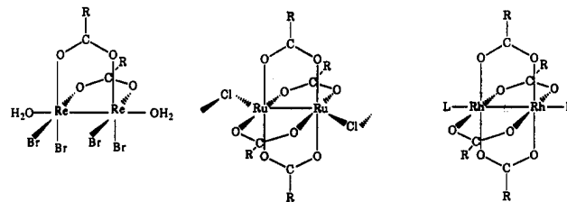
Scheme 1. Molecular Drawings of the Three Structural Types Encountered for Dinuclear Carboxylate Compounds That Exhibit Carcinostatic Activity
